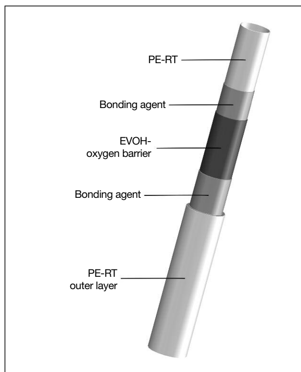
“Copert” PE-RT plastic pipe
